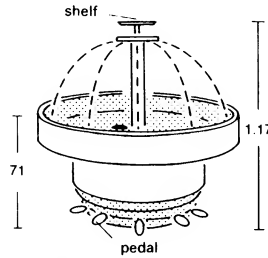
④ Washing fountain (gives 25% space saving over rows of wash-basins → ② + ①)
